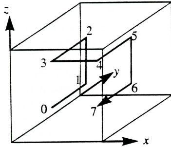
Figure 11. Order of the eight subcubes.
