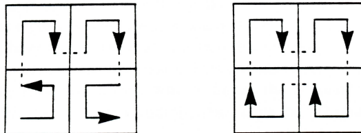
a) Hilbert's curve.
