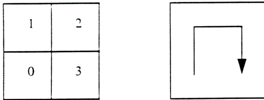
Figure 9. Ordering of the four subsquares.
