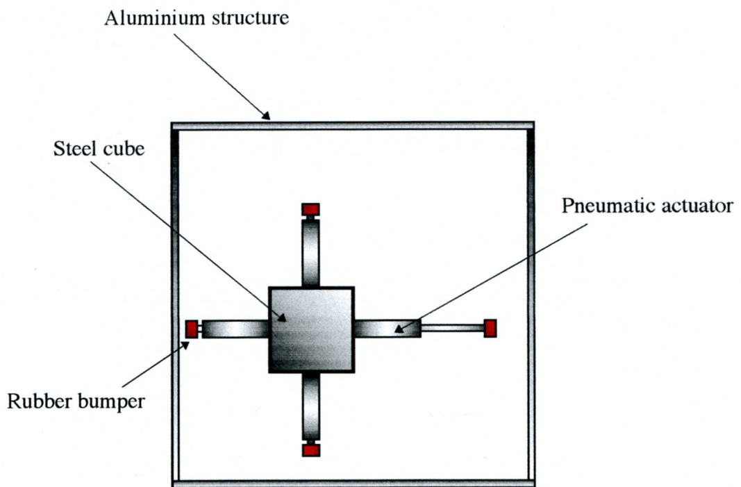
Inverted Scavengers - top view of the installation.
