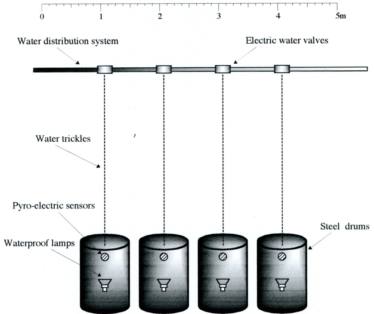
The Flaunted - robotic installation schematics.
