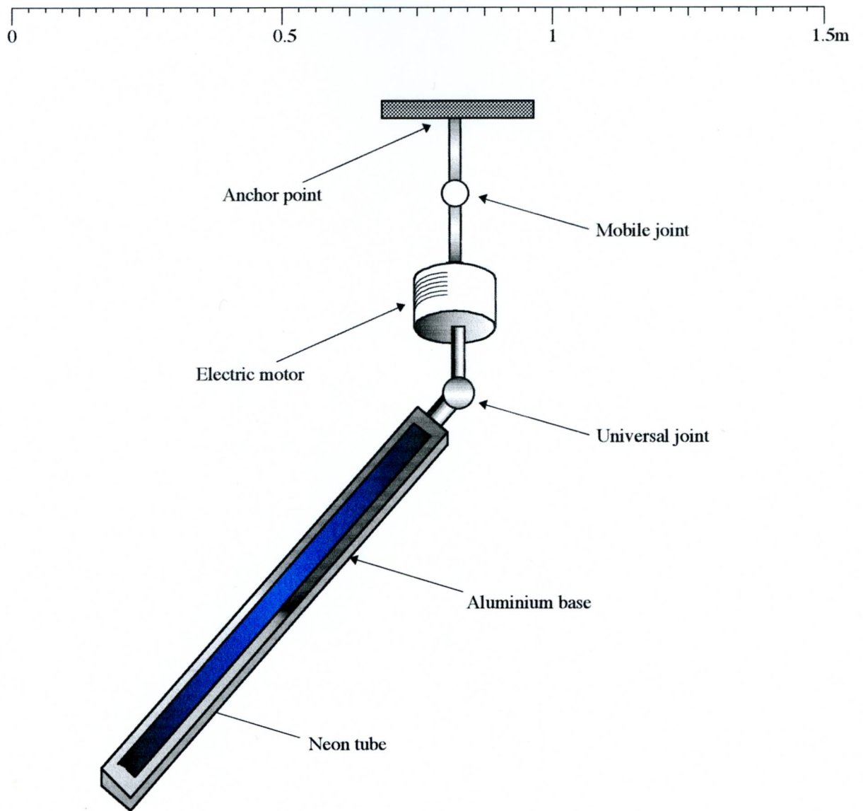
Attractor - side view of robot.
