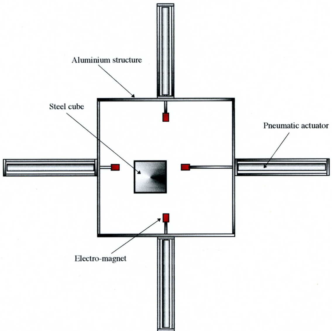
Normal Scavengers - top view of the installation.
