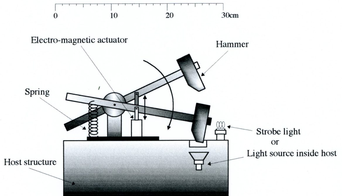
Parasite - robot section.
