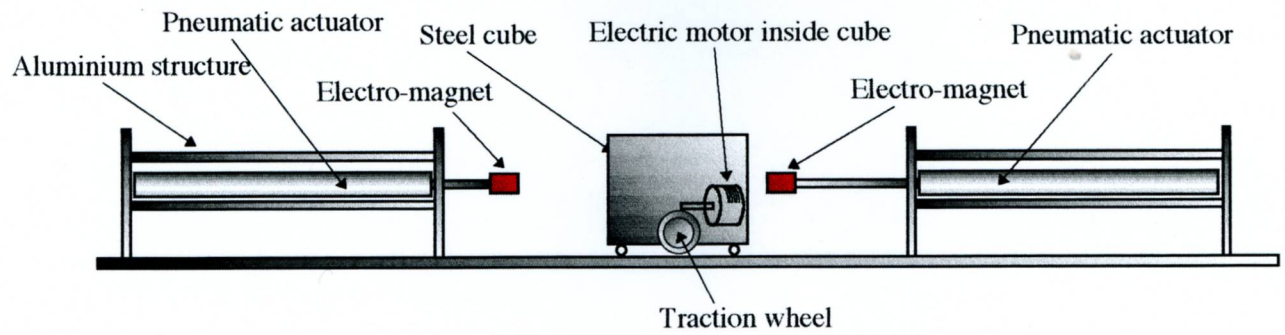
Normal Scavengers - side view of the installation.
