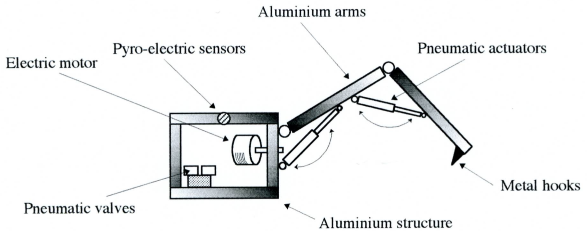
Prisonner - side view of robot.
