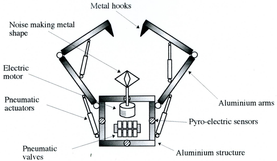
Prisonner - top view of robot.
