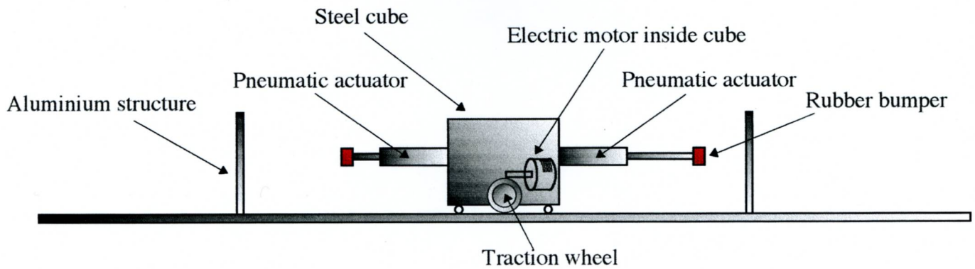
Inverted Scavengers - side view of the installation.
