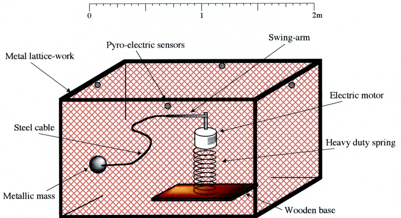
Untamed - robot installation schematics.
