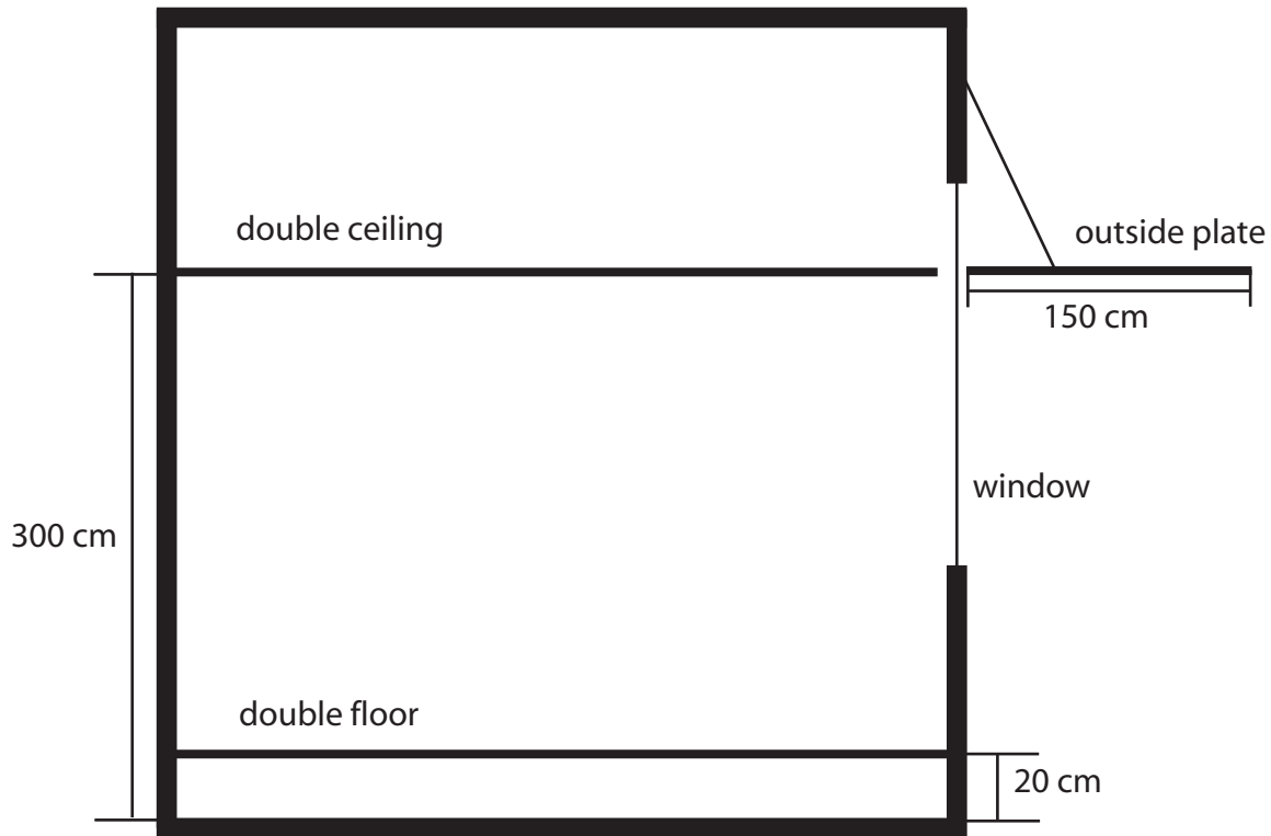
SIDE VIEW
